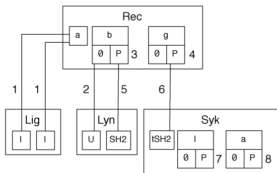
Fig. 2 A contact map for the FcεRI model. 22,23 A contact map shows the molecules, components, and direct binding interactions that are specified in a model. An outer box represents a molecule type. Inner boxes represent components. The possible internal states of components are also represented by boxes below component boxes. Binding partners are connected by lines. This contact map indicates, for example, that the g component of Rec has two possible states (0 and P), and when in the P state, g may bind the tSH2 component of Syk. This component represents the two tandem SH2 domains of Syk. The labels 1, 2, 5 and 6 refer to sets of rules in the FcεRI model 22,23 that characterize association/dissociation reactions. The labels 3, 4, 7 and 8 refer to sets of rules that characterize internal state change reactions, i.e. , phosphorylation reactions in the FcεRI model. 22,23 All of these rule sets are described in Appendix S1 (ESI†).
