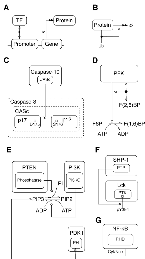
Fig. 6 Visualization of various cell signaling processes. (A) Stimulation of transcription and translation by transcription factor (TF) binding to DNA. (B) Stimulation of protein degradation by ubiquitination. (C) Proteolysis. Dotted box lines identify the parts of the caspase-3 polypeptide chain affected by the proteolytic action of caspase-10. Cleavage of the indicated peptide bond breaks the chain itself and the CASc segment. (D) Allosteric regulation of a metabolic reaction, conversion of F6P (fructose 6-phosphate) to F(1,6)BP (fructose 1,6-bisphosphate). The effector is F(2,6)BP (fructose 2,6-bisphosphate). (E) Lipid phosphorylation and dephosphorylation, and PH domain interaction with phosphatidylinositol (3,4,5)-trisphosphate (PIP3). The small-molecule metabolites ATP and ADP and inorganic phosphate ( P_i ) are shown to participate in the reactions between phosphatidylinositol (4,5)-bisphosphate (PIP2) and PIP3 to illustrate how such details can be represented in a map if desired. However, such details would normally be omitted for simplicity. (F) Protein dephosphorylation. (G) A protein (NF- \kappa B) that traffics between the cytoplasm (Cyt) and nucleus (Nuc).
