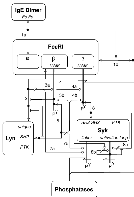
Fig. 3 A molecular interaction map for the FcεRI model. 22,23 A MIM illustrates molecules, reactions, and contingencies. A line that begins and ends with an arrowhead represents noncovalent binding, whereas a pair of parallel lines with no arrowheads represents covalent binding. An open circle indicates enzymatic catalysis, an open triangle indicates stimulation, and a jagged line indicates cleavage of a covalent bond. For additional information about MIM conventions, see Kohn et al. 66,68 The numbers 1–8 refer to sections of Appendix S1 (ESI†). Annotation of this MIM is provided in Appendix S2 (ESI†). Note that this MIM is intended to be read using the combinatorial interpretation of MIM notations. 66
