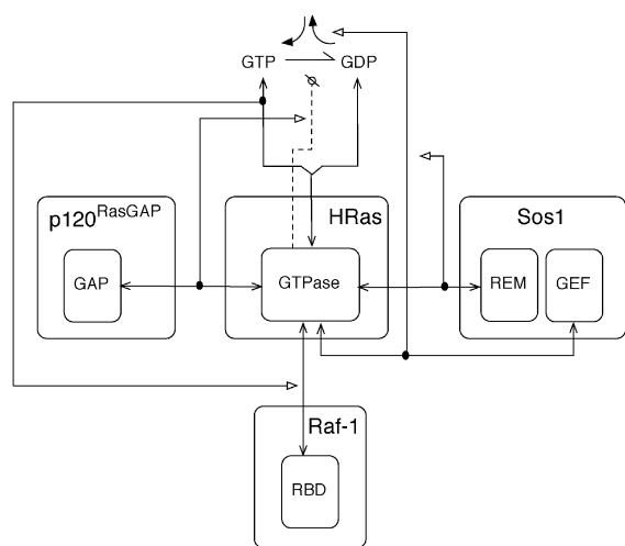
Fig. 8 Visualization of Ras regulation. HRas, which has GTPase activity, is drawn with branched arrows pointing to GTP and GDP to indicate that HRas contains a single binding site for the guanine nucleotides. The reaction arrow between GTP and GDP represents the transition from one bound state of GTPase to another. A catalysis arrow is drawn from the GTPase domain of HRas to the GTP-to-GDP reaction arrow to represent the intrinsic catalytic activity of HRas. The arrow is dotted to indicate that it represents a cis interaction ( i.e. , the GTPase acts on a GTP molecule that is bound to itself). A stimulation arrow is drawn from the GTPase-GAP interaction arrow to the catalysis arrow to indicate GAP-mediated upregulation of GTPase activity. Exchange of GDP for GTP is represented with a pair of bent arrows, and an activation arrow indicates that Sos1 stimulates exchange. Sos1 is allosterically activated by HRas binding to the REM domain.
