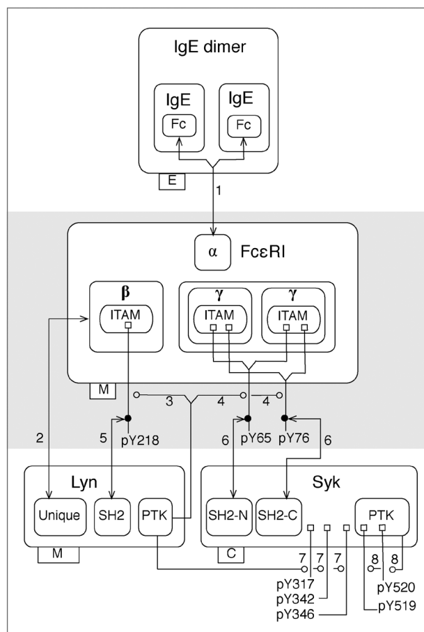
Fig. 4 An extended contact map for the FcεRI model. 22,23 Molecules are represented with nested boxes. A direct physical interaction is represented by an arrow that begins and ends with an arrowhead. An enzyme–substrate relationship is represented by an arrow that begins at an enzyme or catalytic subunit box and terminates with an open circle, which identifies the substrate. Tags attached to lower left corners of molecule boxes identify compartmental locations: E stands for extracellular, M stands for plasma membrane (the subunits of FcεRI are transmembrane proteins and Lyn is anchored to the inner leaflet of the plasma membrane), and C stands for cytoplasmic (Syk is able to freely diffuse in the cytoplasm). Phosphatase activity is not depicted in this map, as phosphatases are considered only implicitly in the model. 22,23 Note that Arrow 5 corresponds to the rule of eqn (1) and Fig. 1. The labels 1–8 next to arrows refer to sections of Appendix S1 (ESI†). Each section includes a summary of available knowledge about an interaction and a set of rules that formally characterize the interaction. Note that the numbered arrows in this diagram correspond to the numbered lines/arrows in the diagrams of Fig. 2 and 3.
