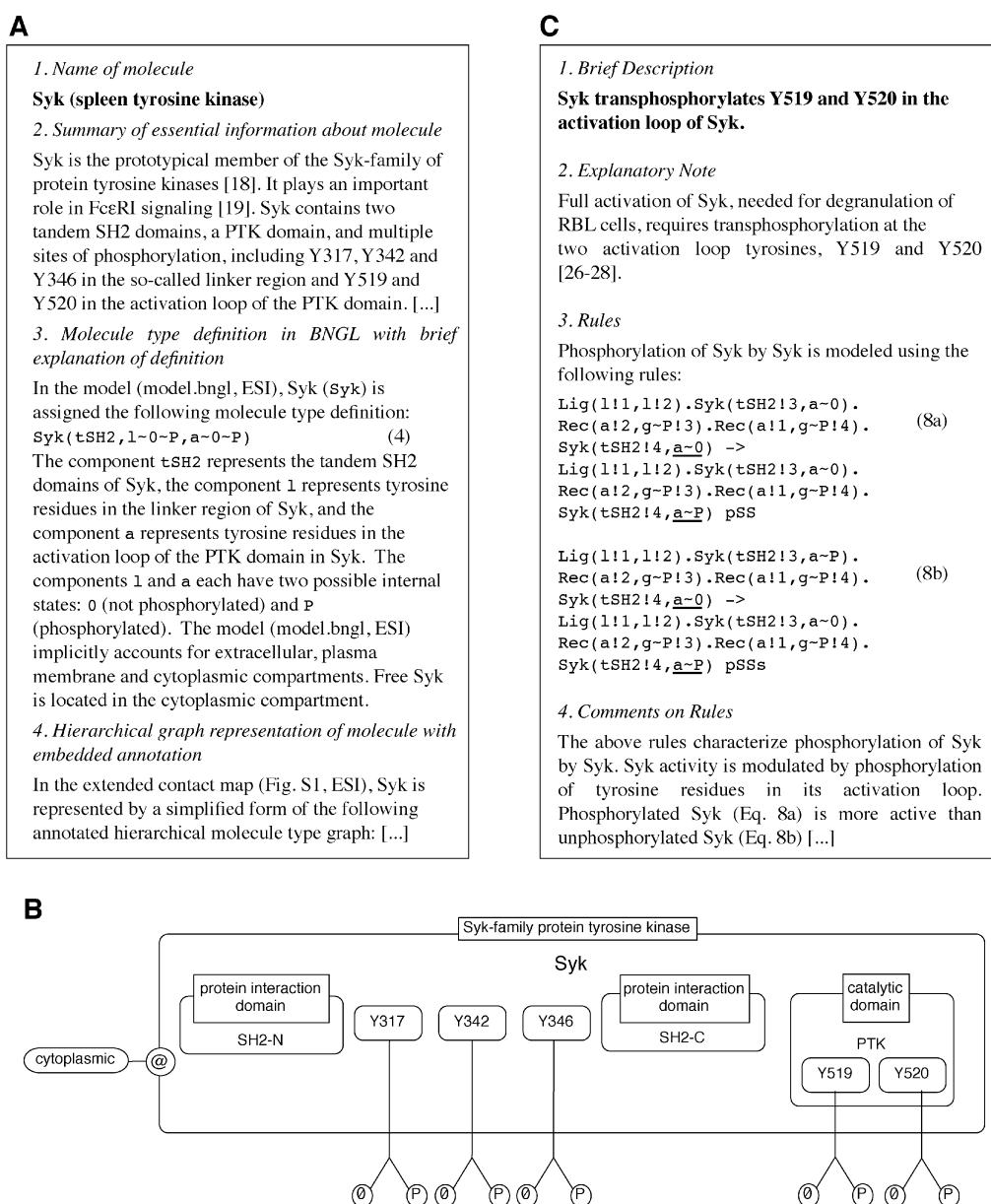
Fig. 10 Excerpts from the model guide of Appendix S1 (ESI†). (A) A protein annotation includes the name of a protein, a molecule type definition in BNGL, and a summary of relevant information from the literature. Other information may be included as well, such as a UniProt accession number ( http://uniprot.org ) and experimental data. (B) Illustration of Syk with embedded annotation. This panel demonstrates how an ad hoc illustration of a molecule can be included in a guide to supplement a standardized representation of a molecule in a map. (C) An interaction annotation includes a brief description of the interaction, a listing of all rules that characterize the interaction, and an explanation of modeling assumptions.
