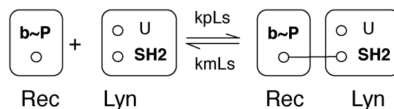
Fig. 1 Visualization of the rule of eqn (1). A molecule or part of a molecule is represented as a set of vertices, which represent molecular components. Vertices are labeled and may also be attributed. Here, the vertex b has the attribute P . Bonds are represented as edges. The reaction center defined by this rule is highlighted by bold vertex labels.
