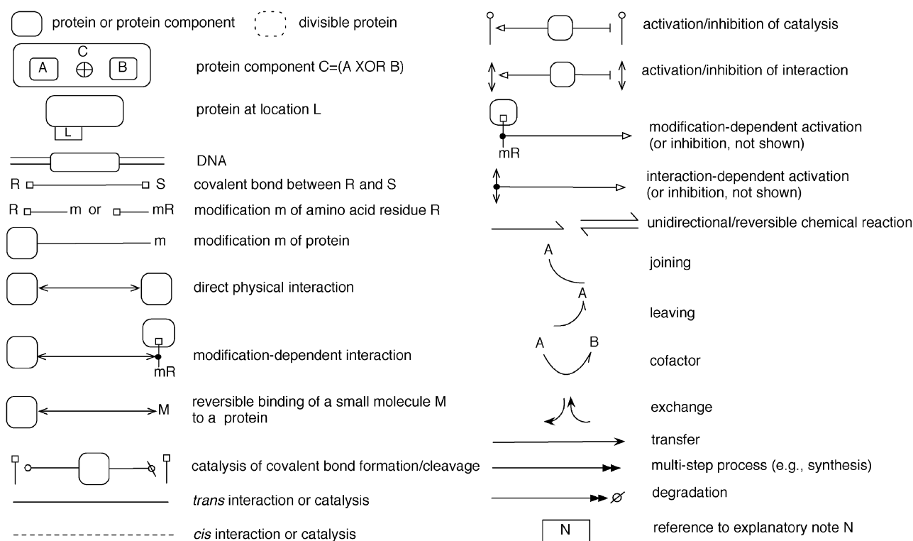
Fig. 5 Boxes, flags, arrows and other symbols that can be used to draw an extended contact map. All of these glyphs are used in example diagrams that follow; see the main text for discussion. The label 'm' represents a post-translational modification. A separator, such as ':', can be inserted between the two parts of a modification flag label. Thus, 'mR' and 'm:R' are both acceptable forms of a modification flag label. For post-translational modifications commonly involved in cell signaling, 73 we recommend the following labels: Ac for acetylation, Me for methylation, OH for hydroxylation, p or P for phosphorylation, and Ub for ubiquitination. The 'joining,' 'leaving,' and 'cofactor' arrows are intended for use in combination with chemical reaction arrows. Note that the joining and leaving arrows together equal a cofactor arrow. In the ESI†, the glyphs shown here are available electronically in the form of an OmniGraffle stencil package (Contact Maps.stencil). OmniGraffle is a general-purpose drawing tool that is commercially available for the Mac platform (The Omni Group, Seattle, WA). The ESI† also contains instructions for use of the stencil package (see README.txt). Updates of the stencil package will be made available at the BioNetGen web site ( http://bionetgen.org ).
